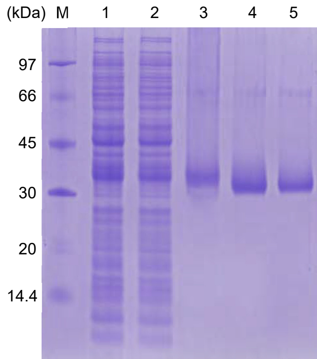
S2 Fig. Expression and purification of recombinant MERS-CoV M pro .
