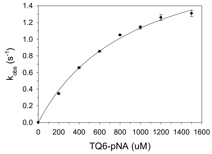
S4 Fig. Activity assay of SARS-CoV M pro .
