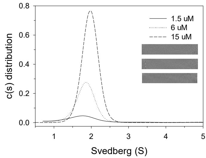
S5 Figure. Continuous size distribution of MERS-CoV M Pro at various protein concentrations.
