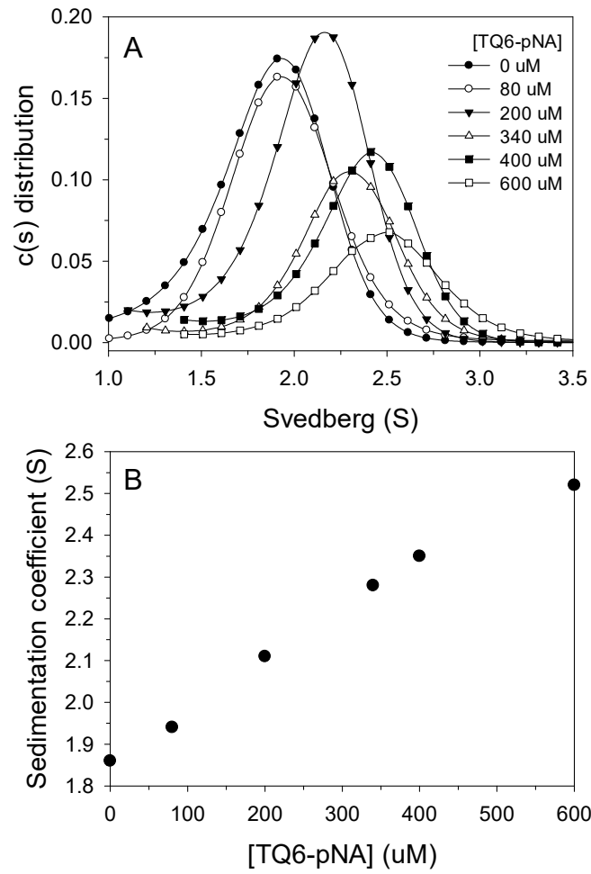
S6 Figure. Effect of substrate concentration on the dimerization of MERS-CoV M pro .
