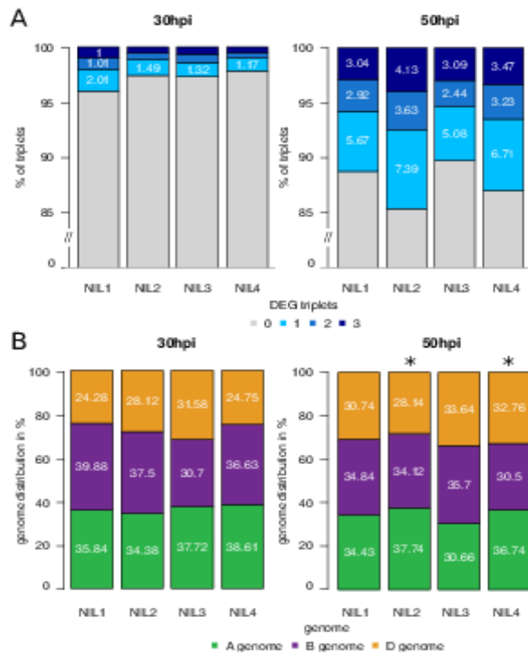
Supplemental Figure 10 - Analysis of triplet expression. (A) Ratio of differential expressed triplet members. (B) Subgenome distribution of triplets with only one members showing differential expression after treatment with Fusarium graminearum . Significance of deviations from the expected distributions was quantified by a chi-squared test against 10,000 random multinomial distributions following the expected A, B, D subgenome distribution from the bread wheat high confidence gene set (* FDR adjusted P < 0.05 ).
