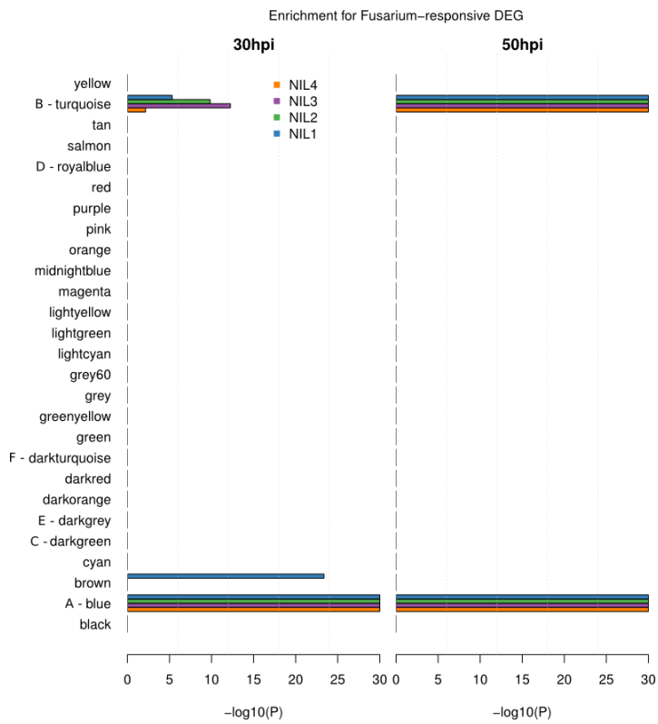
Supplemental Figure 3 - Enrichment for differentially expressed genes within the co-expression modules. FDR adjusted P values from a one-sided Fisher's exact test. For readability the bars were truncated at 10-30. Color names refer to the original WGCNA module labeling.
