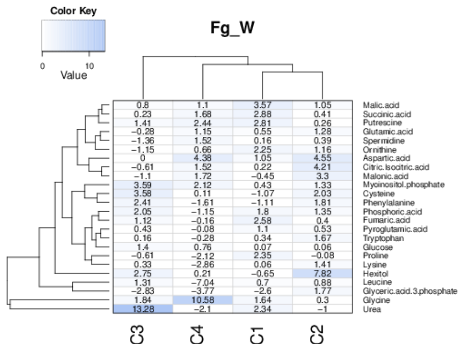
Supplemental Figure 4 - Scoring of the differences in treatment for the comparison between DON and water treatment on the metabolomics data.
