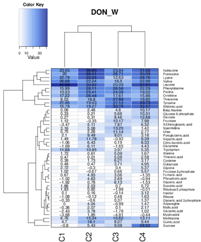
Supplemental Figure 4 - Scoring of the differences in treatment for the comparison between DON and water treatment on the metabolomics data.
