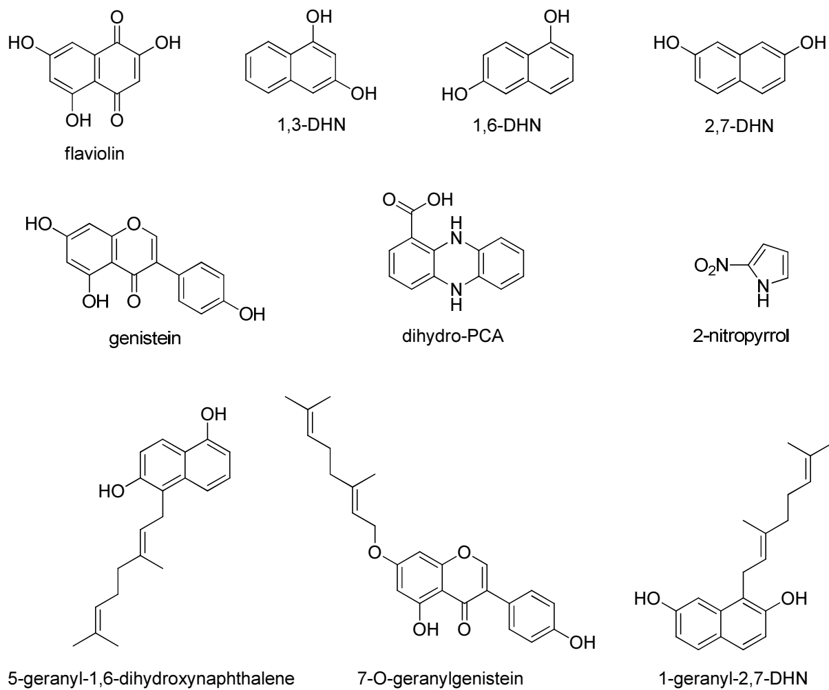
S1 Fig. Aromatic substrates used for prenyltransferase assays and predicted products.
