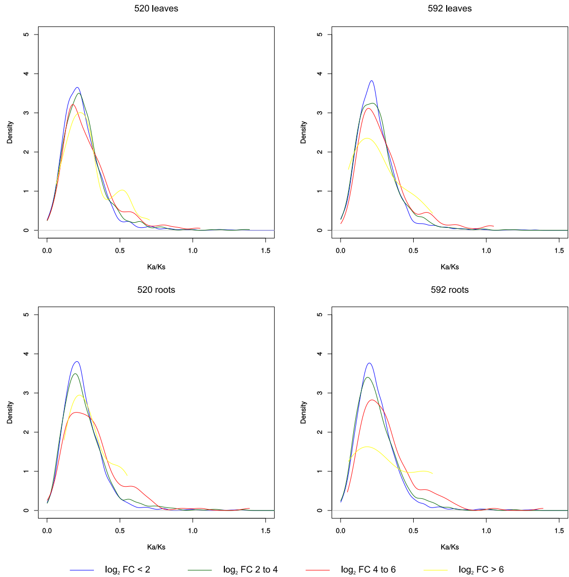
Figure S1. Ka/Ks ratios of Salicoid duplicates classified based on level of differential expression.
