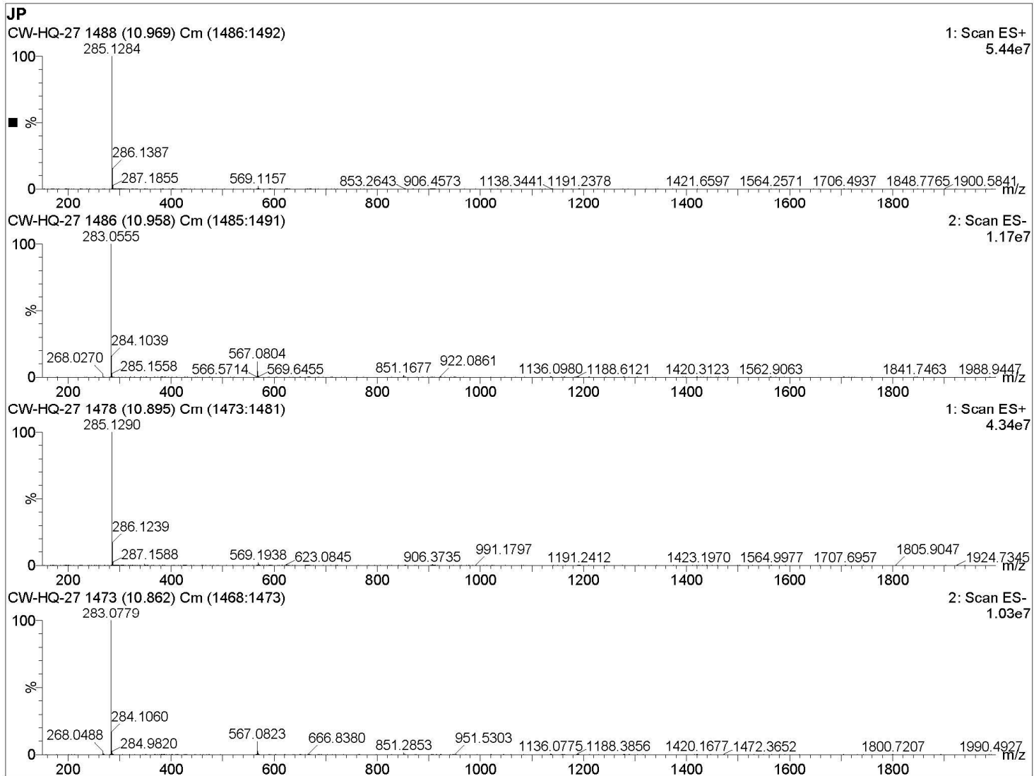
Figure S3. LC-MS spectrum of calycosin.
