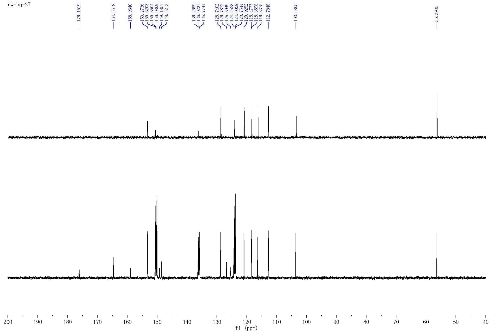
Figure S2. ^{13}\text{C} -NMR (100 MHz, pyridine- d_5 ) spectrum of calycosin.
