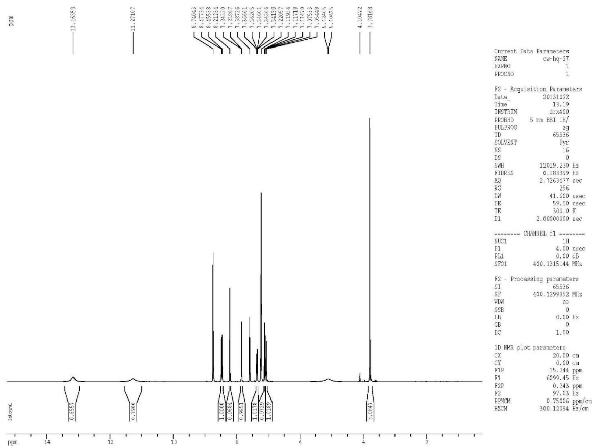
Figure S1. 1 H-NMR (400 MHz, pyridine-d 5 ) spectrum of calycosin.
