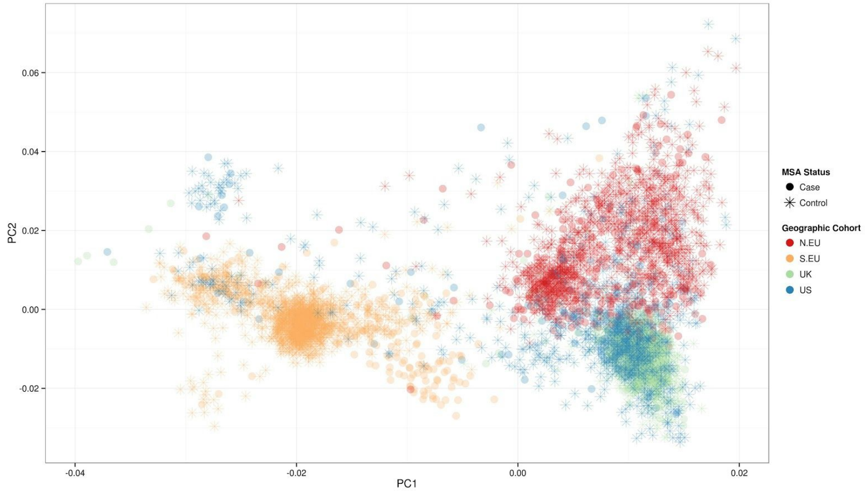
Figure S1: Population stratification using the top two principal components from genotyped SNPs demonstrates that MSA cases and controls cluster together with respect to their geographic cohort.
