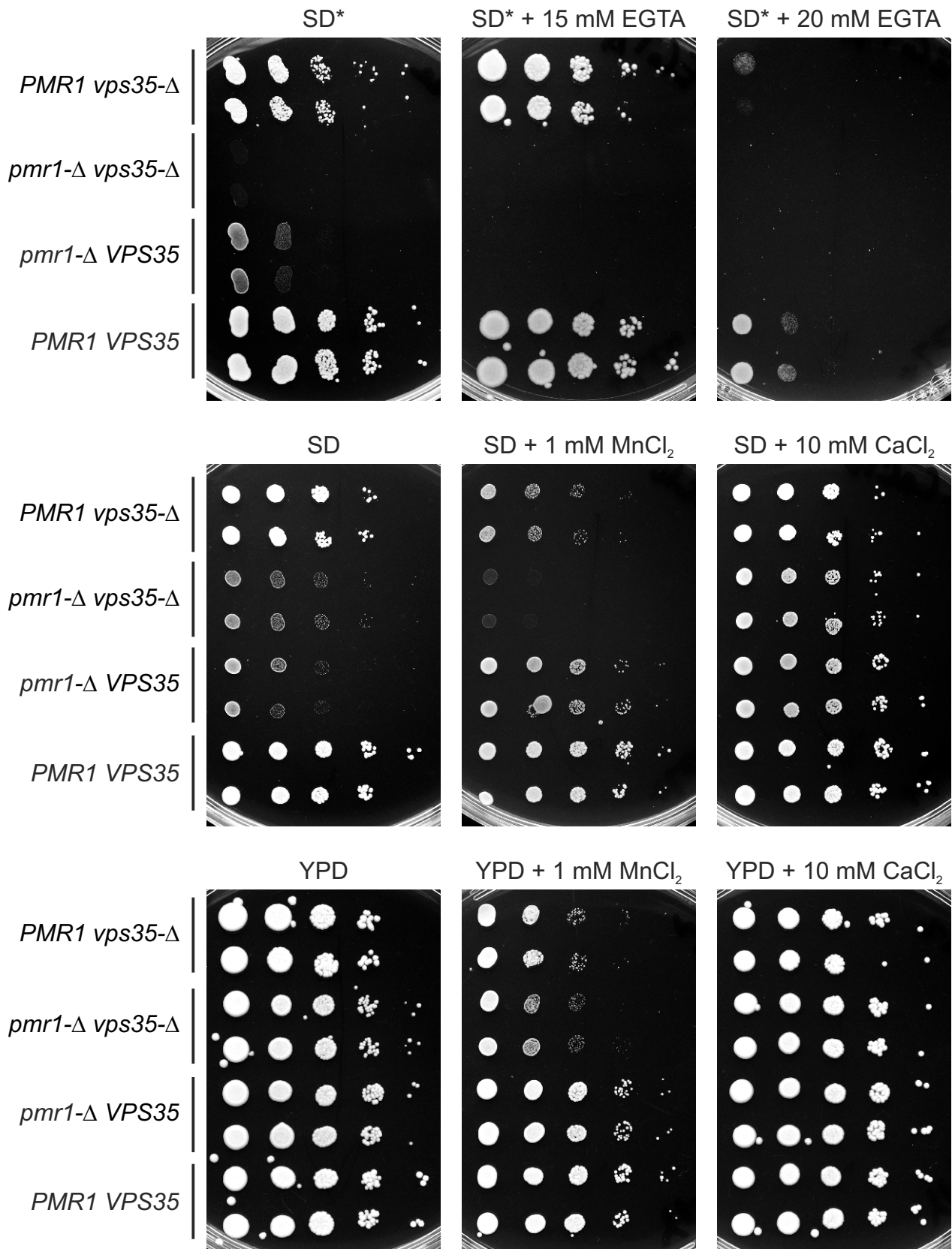
S6 Fig. Effect of the vps35-Δ mutation on growth of strains with or without the PMR1 gene. Cell suspensions with equal densities were serially diluted (10-fold) and spotted onto corresponding media. Two subclones of each strain were analysed. pmr1-Δ vps35-Δ , 1MA27/12/GP1-Δ vps35 strain lacking the plasmid with PMR1 ; vps35-Δ , 1MA27/12/GP1-Δ vps35 strain, pmr1-Δ VPS35 , 1MA27/12/GP1 strain lacking the plasmid with PMR1 ; PMR1 VPS35 , 1MA27/12/GP1 strain.
