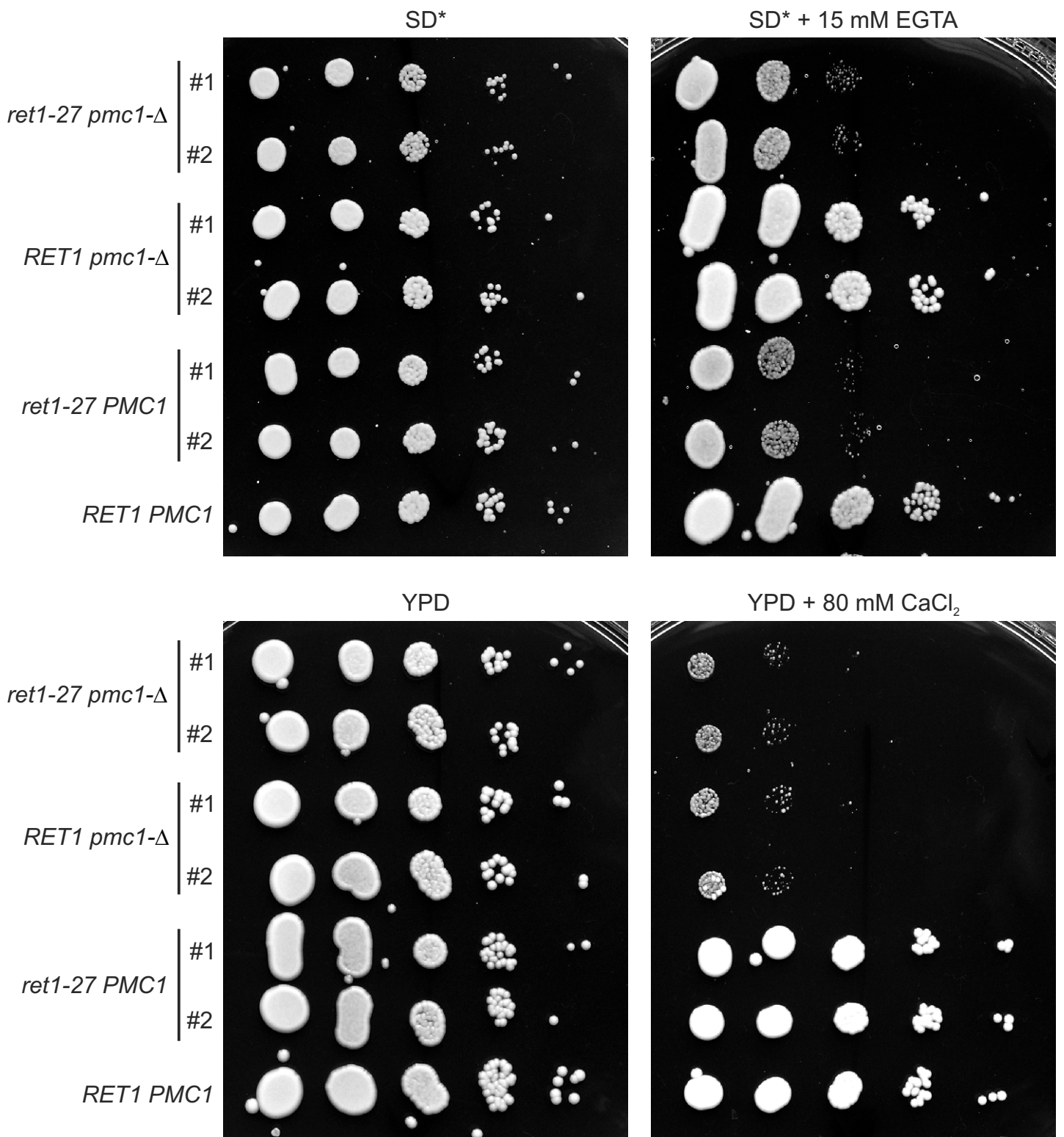
S7 Fig. Sensitivity of the ret1-27 pmc1-Δ double mutant to a shortage (achieved by addition of EGTA) or excess of Ca 2+ in culture medium. Cell suspensions with equal densities were serially diluted (10-fold) and spotted onto corresponding media. The replication of this experiment with additional concentrations of Ca 2+ and EGTA is shown in Fig. 5. ret1-27 pmc1-Δ , 64MA70QA-Δ pmc1 strain; pmc1-Δ , 64MA70Q-RET-Δ pmc1 strain; ret1-27 , 64MA70QAL strain; RET1 PMC1 , 64MA70QL-RET strain; #1 and #2, independently obtained clones.
