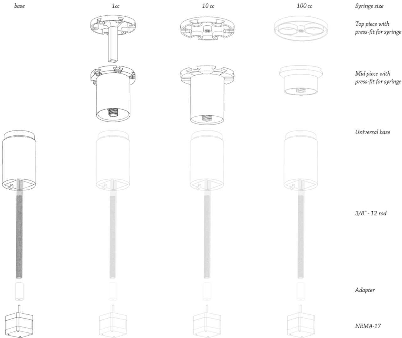
Fig. S8 | Modular components of the syringe pump. (Left) The base of the pump includes the Nema 17 stepper motor, a 3D printed connector, and the 3D printed base. The motor press fits into the 3D printed base. The 1cc configuration was used in the DNA assembly experiments. The Mid & Top pieces were modified to accommodate 10 and 100cc syringes.
