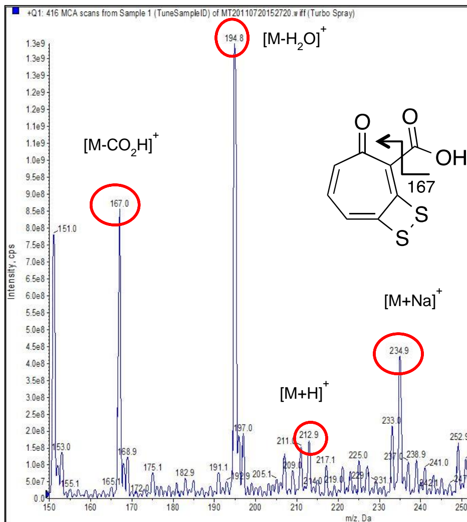
Additional File 1. Electrospray ionization MS of purified TDA, structure shown on right, in the positive ion mode. The spectrum shows expected losses of H 2 O and CO 2 H.
