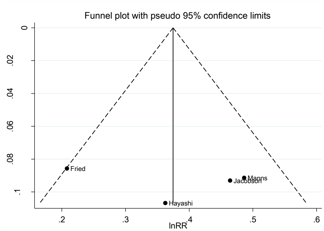
S3 Figure. Funnel plot of risk ratios of sustained virological response at 12 weeks after the end of treatment between simeprevir plus pegylated interferon-ribavirin and pegylated interferon-ribavirin alone
