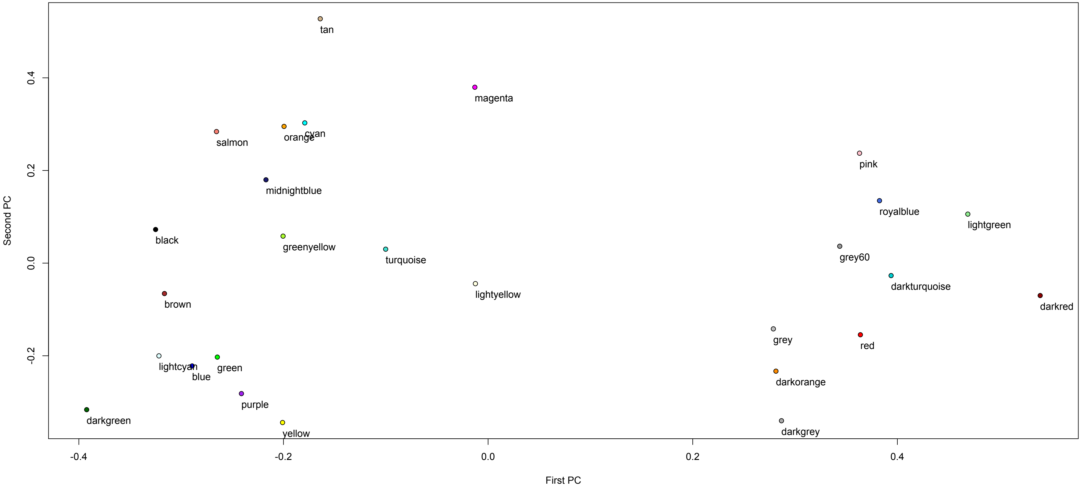
B6Exp1 HPC WGCNA-DS3 Multidimensional Scaling
