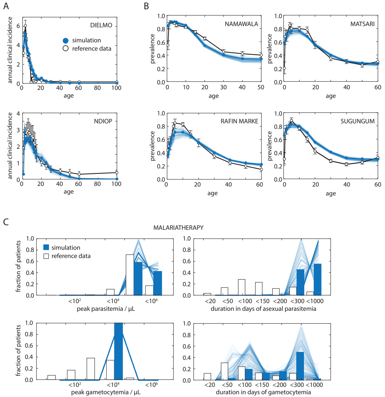
Comparison of incidence, prevalence, peak density, and infection duration between reference data and simulation with calibrated immunity and gametocyte development parameters. Simulation data corresponds to the single (solid blue) and 100 (transparent blue) parameter set(s) with highest combined likelihood across all study sites.
