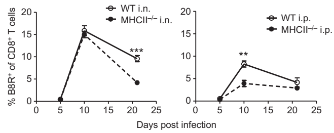
Supplemental Figure 1. Kinetics of B8R-specific CD8 + T cell response in the lungs. WT and MHCII -/- mice were infected with 10 3 PFU of VACV intranasally (i.n.) or intraperitoneally (i.p.). B8R-specific CD8 + T cells were identified by staining with B8R tetramer and anti-CD8 \alpha Ab at the indicated times. Data are representative of two independent experiments with four mice per group. **, p < 0.01 ; ***, p < 0.001 .
