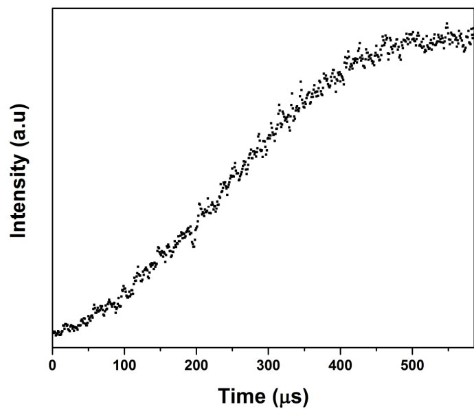
Figure S10. Fluorescence emission rise time of UCNPs. The emission was collected for fluorescence lifetime at 473 nm under 980-nm excitation, showing a rise time of about 310 \mu\text{s} .
