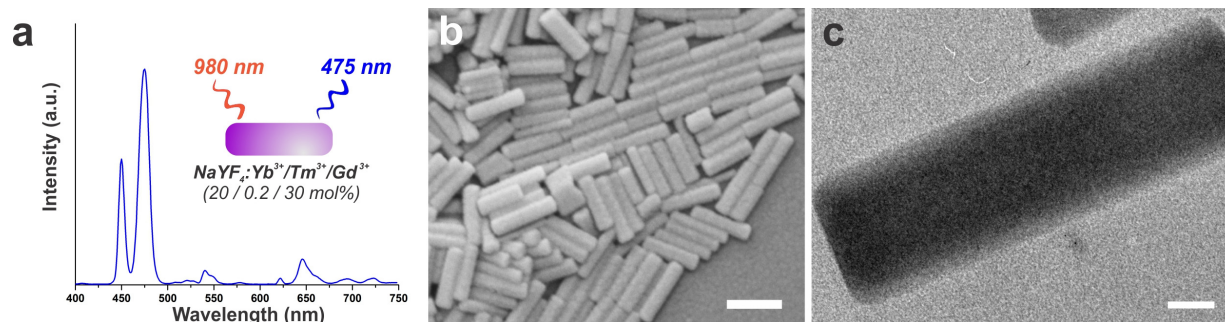
Figure S14. Characterization of blue-emitting upconversion nanorods (UCNRs). (a) Upconversion emission spectrum of the \text{NaYF}_4:\text{Yb}^{3+}/\text{Tm}^{3+}/\text{Gd}^{3+} (20/0.2/30 mol%) UCNRs in hexane solution under laser excitation at 980 nm. (b) SEM image of UCNR. Scale bar: 200 nm. (c) TEM image of UCNR. Scale bar: 20 nm. Both SEM and TEM show a UCNR length of about 200-nm and width of 50-nm.
