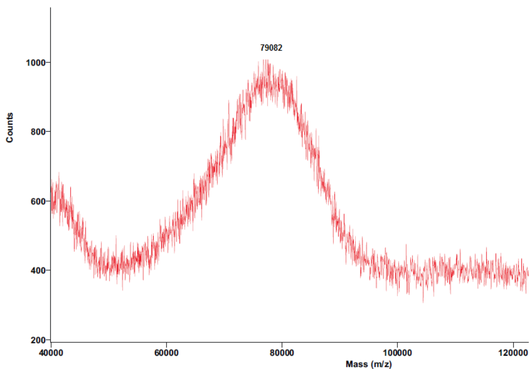
Figure S1: Maldi-tof analysis of (p-SCN-DOTA-4AmPE) [45] conjugated G5 PAMAM dendrimer. The average number of conjugate DOTA-4AmPE chelates was estimated to be 44 per dendrimer.
