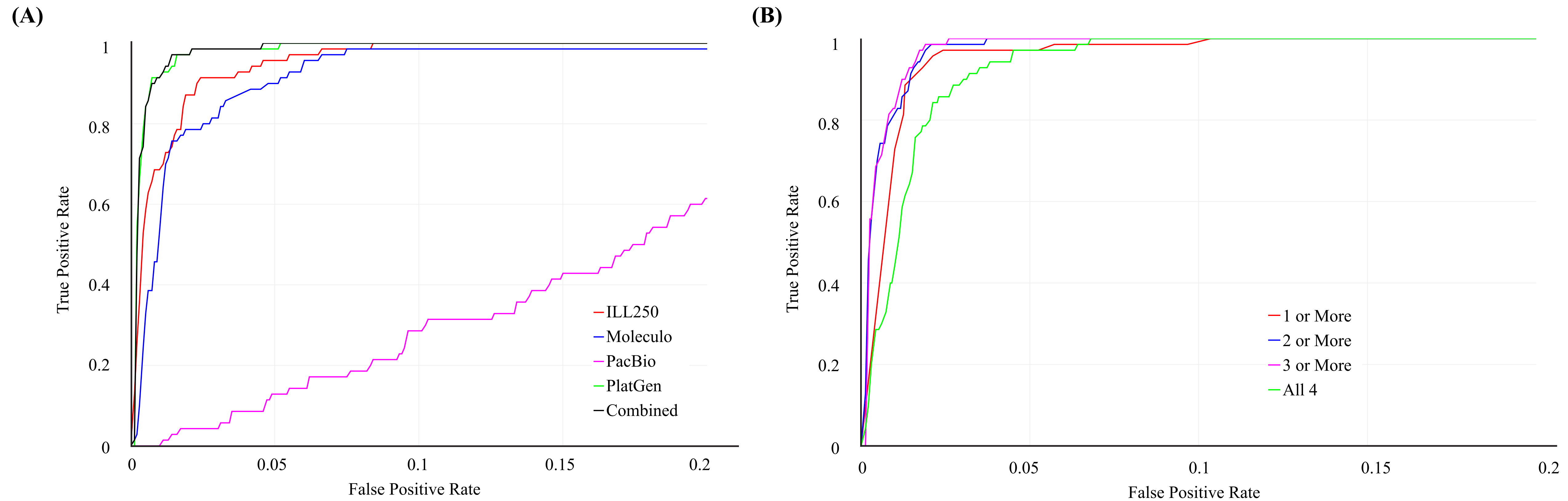
Supplementary figure 5: ROC curves for One-class classification using the L1 Distance, treating the 4000 random regions as negatives and the Spiral Genetics insertions calls as positives. (A) ROC curves for one-class models for each dataset separately and for all combined. (B) ROC curves for one-class model requiring 1 or more, 2 or more, 3 or more, or all 4 technologies to have high classification scores. See original data at https://plot.ly/~desuchen0929/386 , and https://plot.ly/330/~parikhhm/ .
