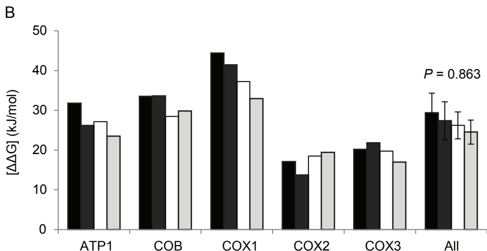
Supplement 3. Changes in thermodynamic stability ( \Delta\Delta G ) between mitochondrial proteins modeled on ancestral and extant Silene sequences, based on (A) relative or (B) absolute \Delta\Delta G .
