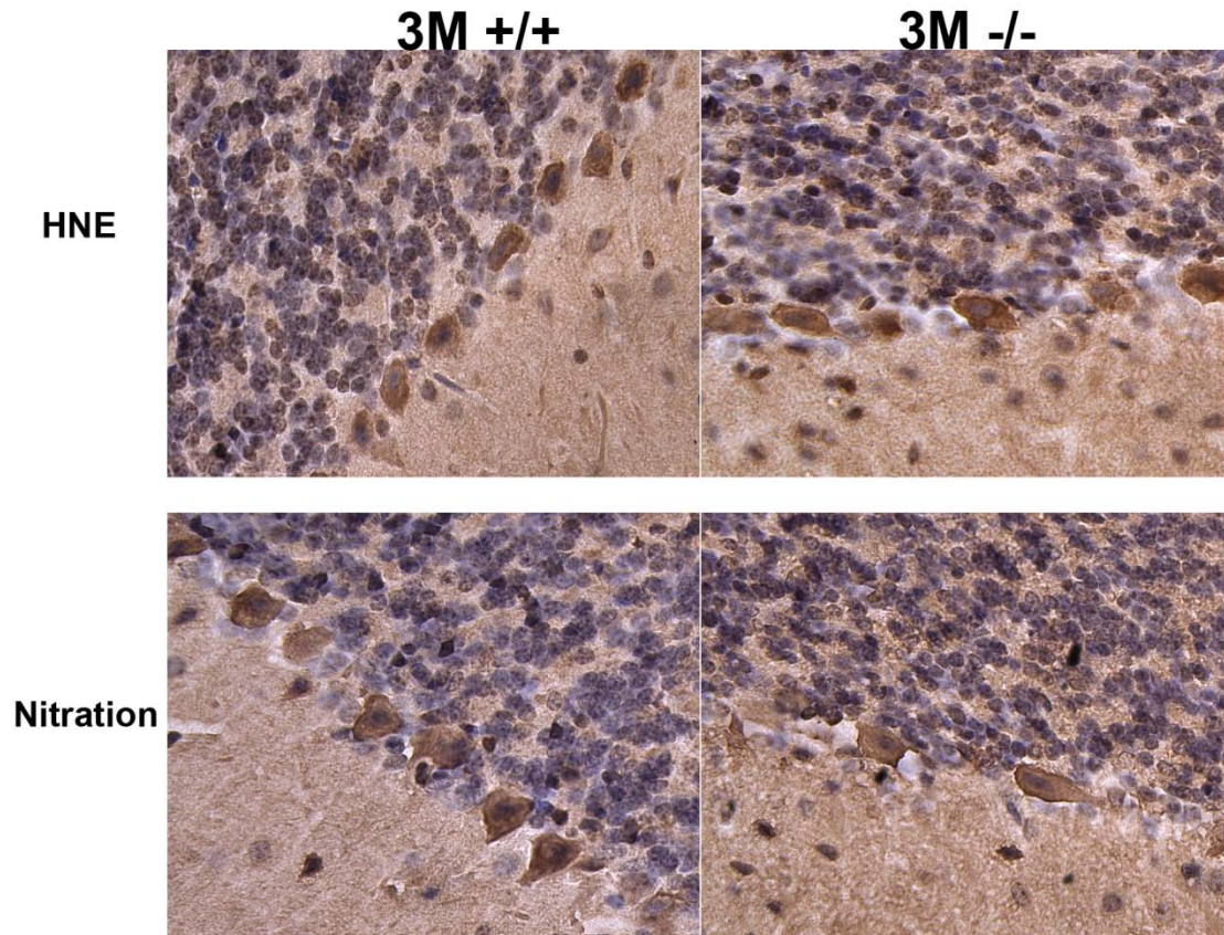
Fig.S1. HNE and nitrotyrosine modification of proteins in young mice. Sections from control and mutant mice were put on the same slide for immunostaining. Color development time was slightly different than for sections of old mice; thus, these images are not directly comparable with images from old mice ( Fig.4B ).
