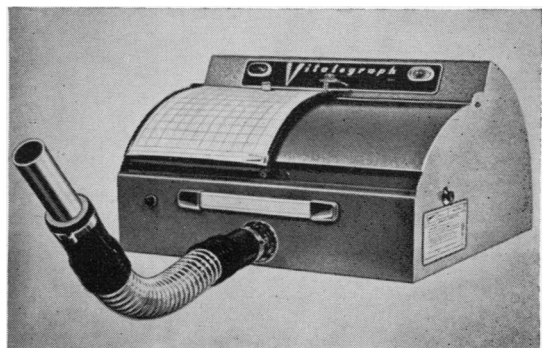
FIG. 1. The Vitalograph spirometer.
