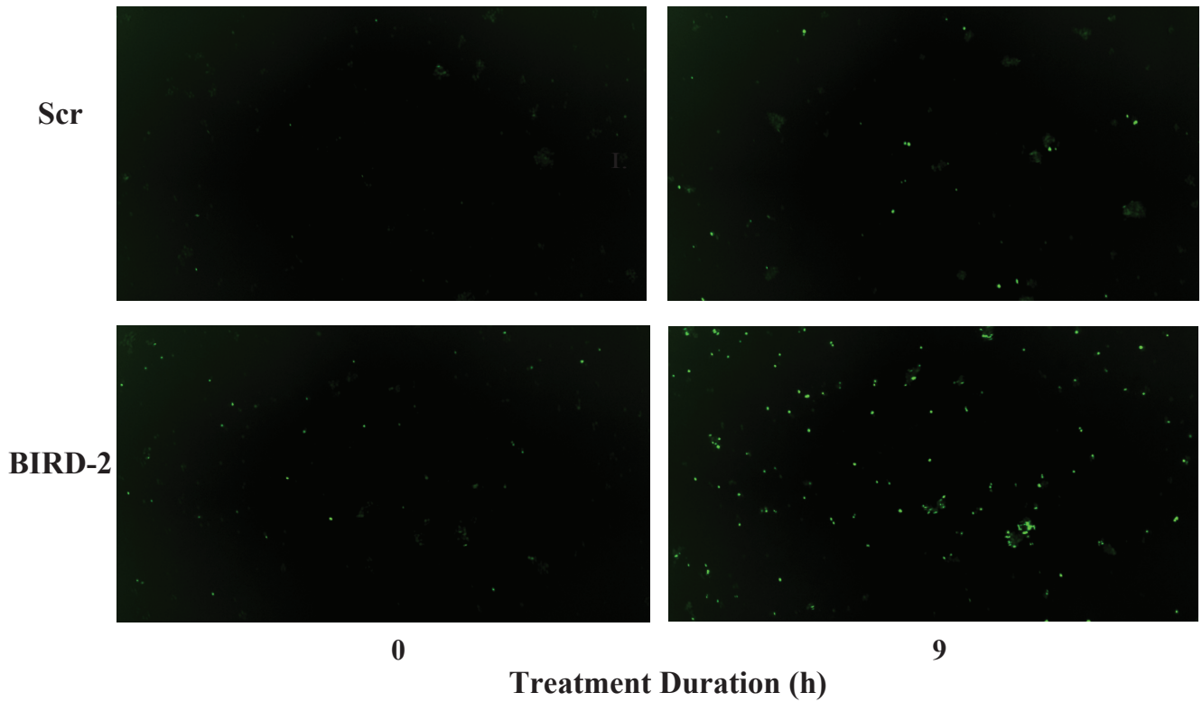
Supplementary Figure 2: Caspase 3/7 activity in SCLC Cells. Representative images obtained from the IncuCyte ZOOM, measuring caspase 3/7 activity in H2171 cells treated with 20 \mu M BIRD-2 or Scr control peptide for the indicated times.
