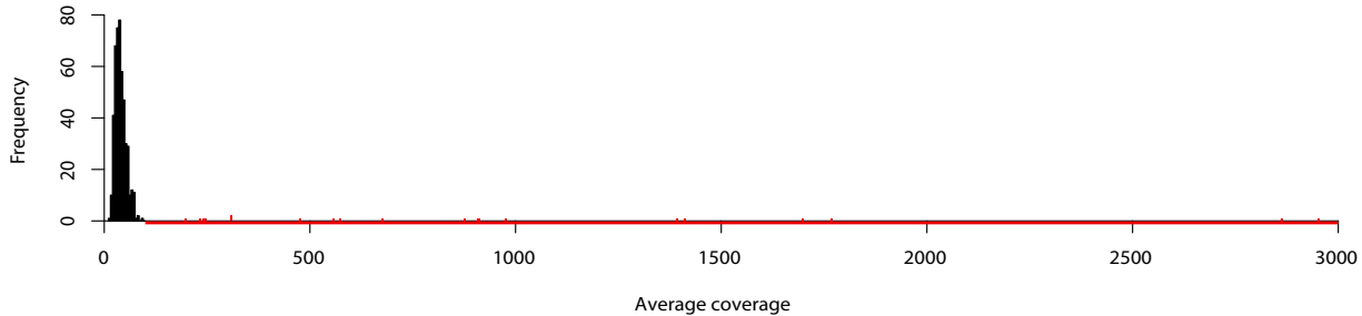
Histogram of average coverage per exon
