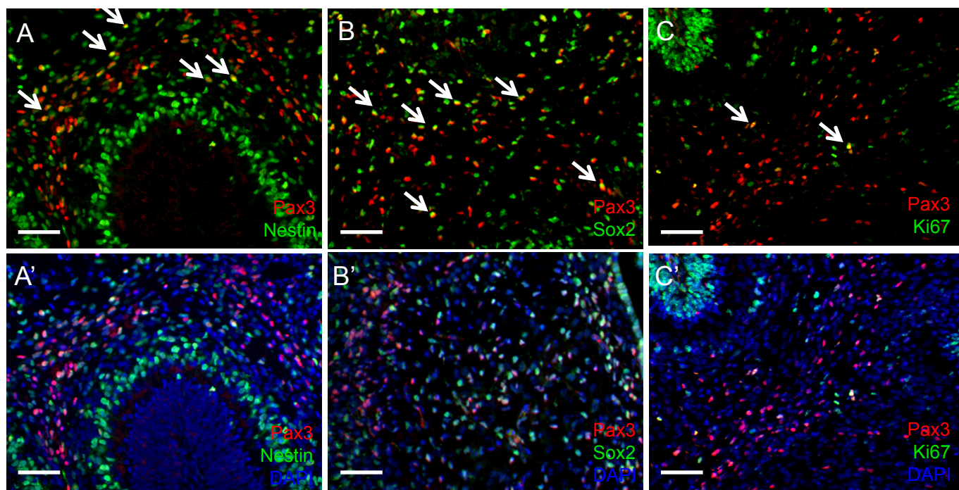
Figure S2. Pax3-expressing cells in the internal granule layer of the cerebellum. Co-immunofluorescence of wildtype P3 mouse cerebellum for Pax3 and Nestin-CFP (using a GFP antibody) (A), Sox2 (B), and Ki67 (C). DAPI counterstain is shown in (A'-C') to indicate total nuclei. 20x magnification, scale bar is 50 \mu m. White arrows point to double positive cells.
