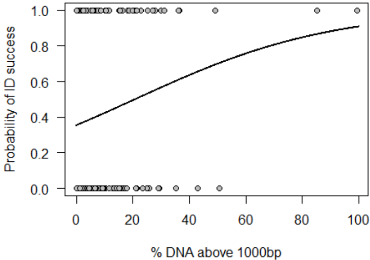
Figure B: The probability of successful ID of a sample as a function of the % of good DNA in the sample.
