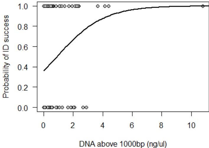
Figure A: The probability of successful ID of a sample as a function of the concentration of good DNA in the sample.
