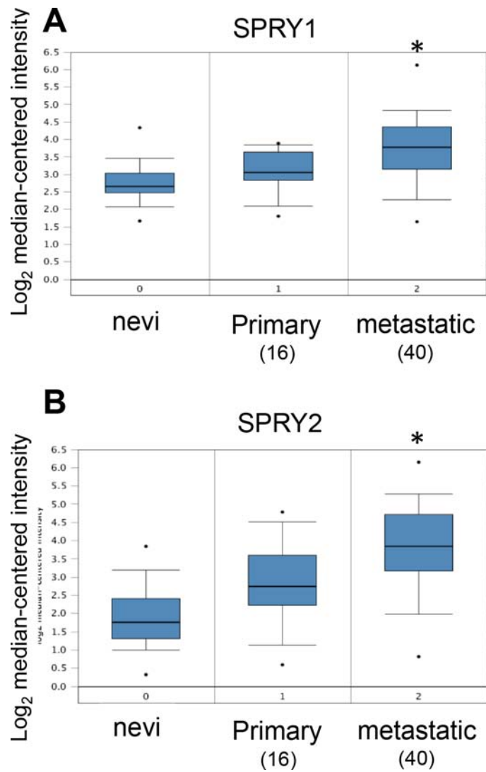
Supplementary Figure S1: SPRY1 and SPRY2 are increased in metastatic melanoma: Riker data set. Expression levels of both SPRY1 and 2 are increased in metastatic melanoma samples versus primary lesions. * p < 0.05 .
