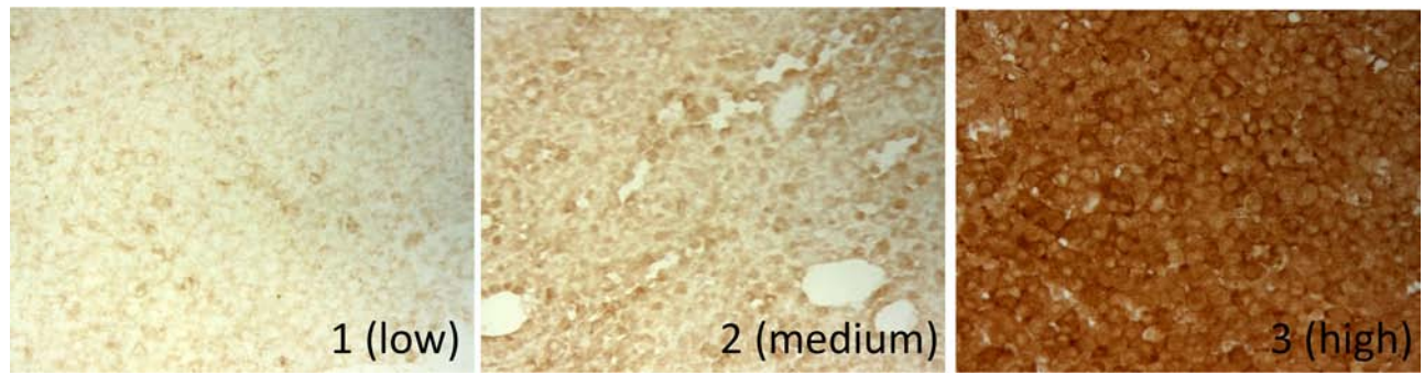
Supplementary Figure S2: staining intensity of the tissue array.
