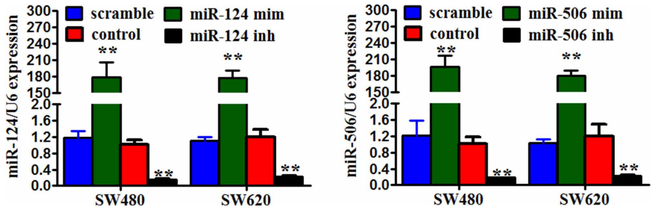
Supplementary Figure S1: The transfection was successful. The transfections of miR-506 mimic, miR-124 mimic, miR-506 inhibitor and miR-124 inhibitor were successful. All data are presented as the mean ± s.e.m., **P < 0.01.
