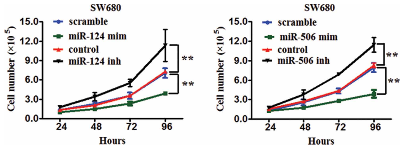
Supplementary Figure S2: The effects of miR-124 and miR-506 inhibitors on tumor cell progression. We found that the miR-124 and miR-506 inhibitors decreased the sensitivity of CRC cells to the two agents. All data are presented as the mean ± s.e.m., **P < 0.01.
