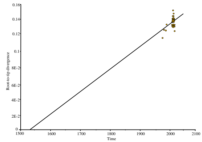
Complete genome
