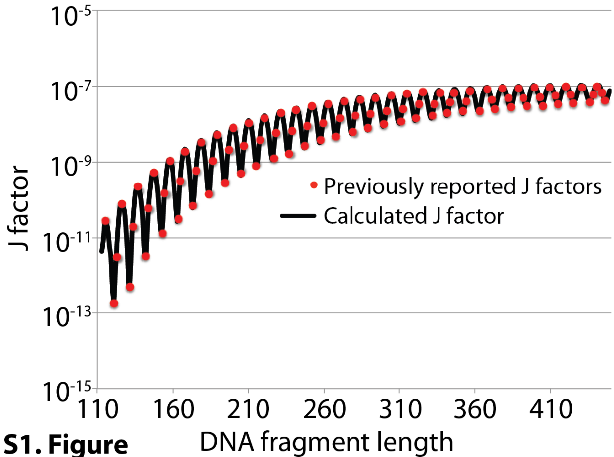
S1. Figure DNA fragment length Figure S1. Validation of the CSO implementation using the model of a straight homogenous DNA sequence. Black line corresponds to calculated J factors, while red circles are used to show J factors based on results reported in ref. (29). The Y-axis depicts J factors (log scaled), while the X-axis reflects the length of the DNA fragment.
