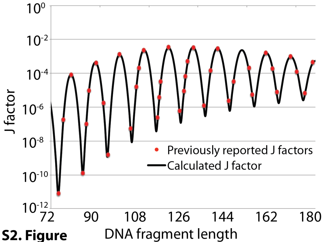
Figure S2. Validation of the CSO implementation using the model of a curved DNA sequence. Black line corresponds to calculated J factors, while red circles are used to show J factors based on results reported in ref. (29). The Y-axis depicts J factors (log scaled), while the X-axis reflects the length of the DNA fragment.
