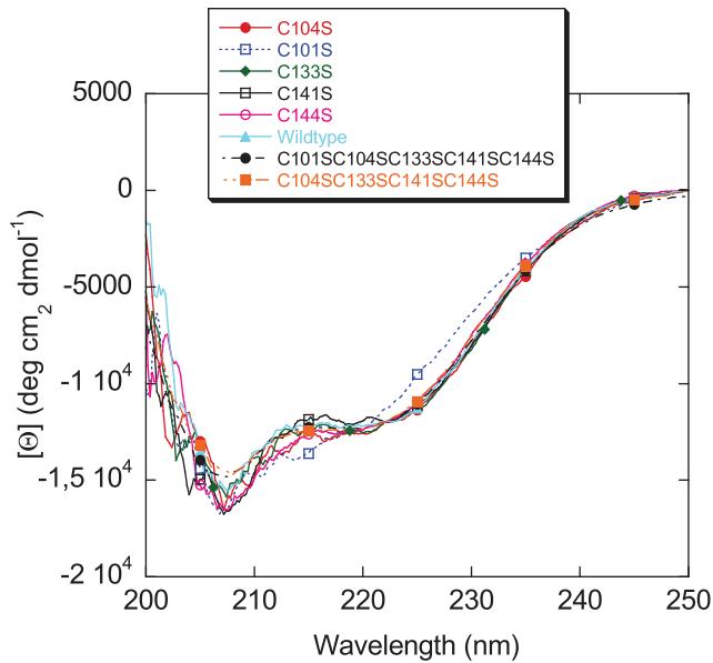
SUPPLEMENTARY FIG. S1. Far UV CD spectra of wild-type FurA and cysteine mutants. The CD experiments were carried out in a Jasco J-815 spectropolarimeter using 0.1 cm cuvettes at 25°C. Spectra were recorded with 10 \mu\text{M} protein solution in 10 mM acetic acid/sodium acetate, pH 4. CD, circular dichroism; Fur, ferric uptake regulator.
