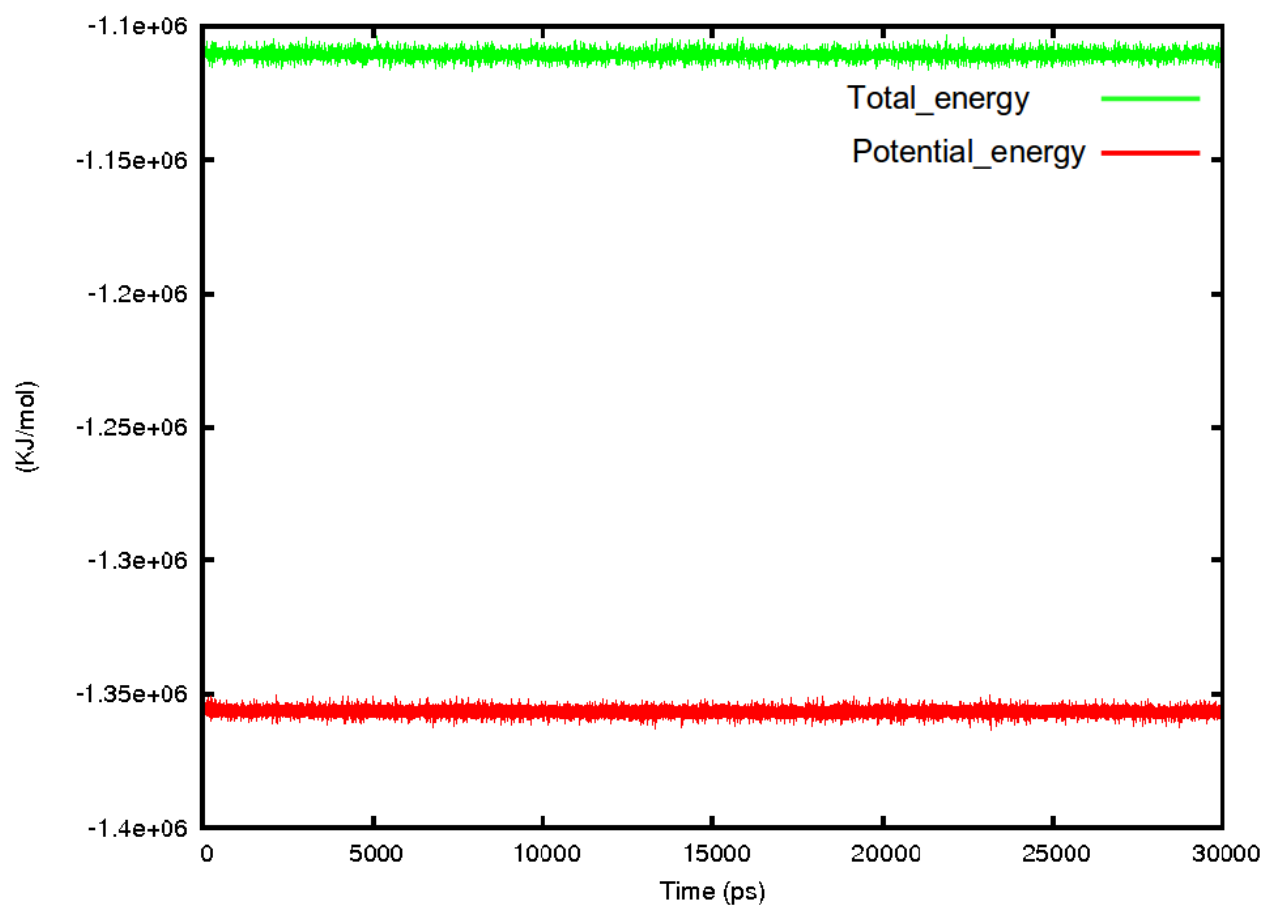
Figure S7 – The variation in total (green) and potential energy (red) for the Rv1712-C5P complex during the 30000ps simulation. Generated using Gnuplotv4.2 [41].
