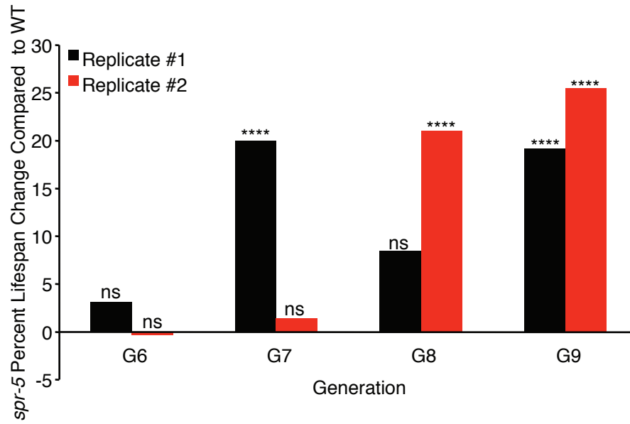
Figure S1: spr-5 mutants display extended transgenerational longevity by generation 7 or 8 Spr-5(by134) mutant worms display a lifespan extension compared to wild type worms by generation 7 or generation 8. Two independent experiments are shown and statistics are presented in Table S1.
