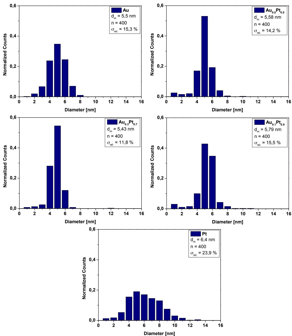
Figure S2. Size distribution of the Au_xPt_{1-x} NP used for catalytic measurements (Polymer: PS(227)-b-2VP(99)).
