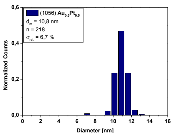
Figure S1. Size distribution of \text{Au}_{0.5}\text{Pt}_{0.5} NP (Polymer: PS(1056)-b-2VP(495)).
