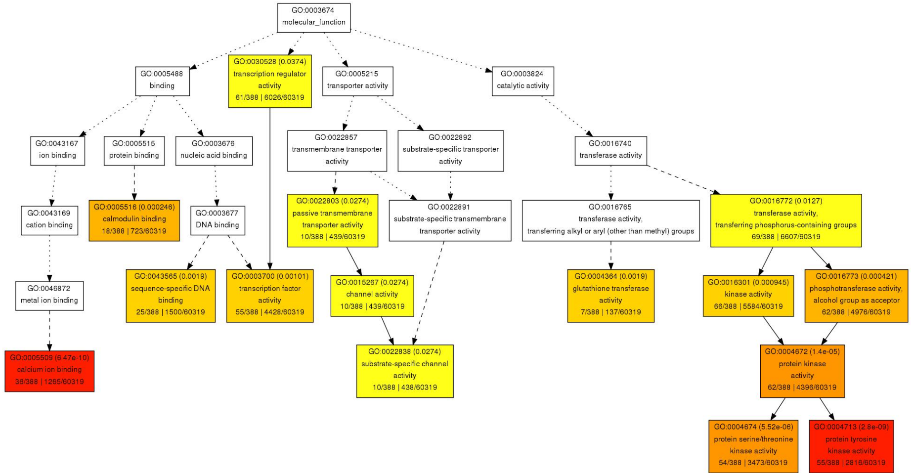
Figure S3. Gene ontology analysis. (a) Molecular Function category enriched GO terms in roots after 30 minutes of water stress. (b) Molecular Function category enriched GO terms in leaf after two hours of water stress. agriGO was employed for analysis and enriched GO terms were obtained using Singular Enrichment Analysis. Colors reflect the level of significance.
