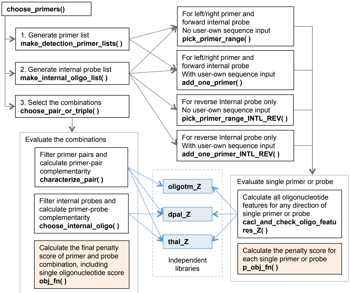
S1 Fig. Schematic structure of Edesign core program.
