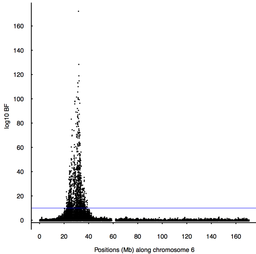
Fig S3. SNP associated with enrichment of African local ancestry in Mexican lipid study. Bayes factors (BF) were computed using BIMBAM. The horizontal blue line is \log_{10} BF = 10 .
