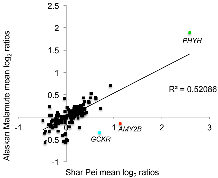
Figure S2. Additional results from analysis of aCGH data. Relationship between Shar Pei and Alaskan malamute mean log 2 ratios for 157 copy number variable sites in the dog genome. GCKR deviates from the null distribution. The location of PHYH likely reflects error in ddPCR measurements due to high copy number.
