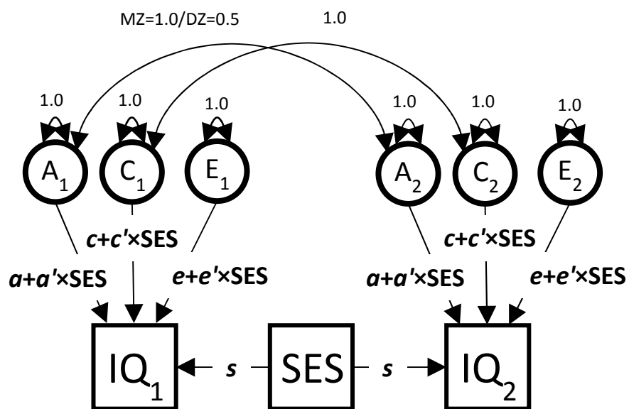
Figure S1. Structural equation model for estimating G \times SES interaction on IQ in twin data.
