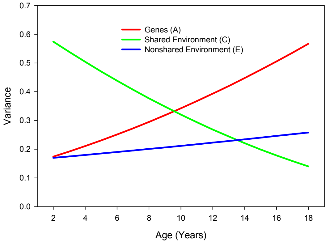
Figure S2. Age trends in genetic, shared environmental, and nonshared environmental variance in cognitive test performance.
