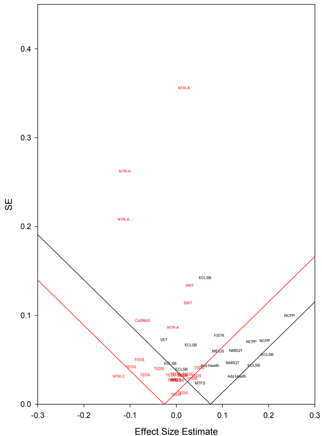
Figure S3. Funnel plot of Gene \times SES interaction effect sizes for US and Non-US Studies, with effect sizes represented by study acronyms (see Table 1).
