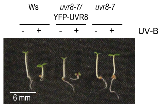
Additional file 4. Overexpression of YFP-UVR8 restores UV-B photomorphogenesis. uvr8-7 seedlings expressing a Pro 35S :YFP-UVR8 construct in Ws background, wild type (Ws) and uvr8-7 mutant seedlings were grown for 4 days under weak white light with or without supplementary UV-B. Images of representative seedlings are shown.
