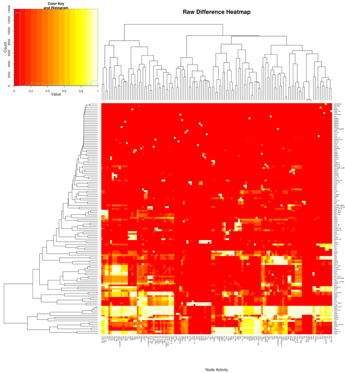
Figure S3: Cell growth condition; inactivating perturbations.
