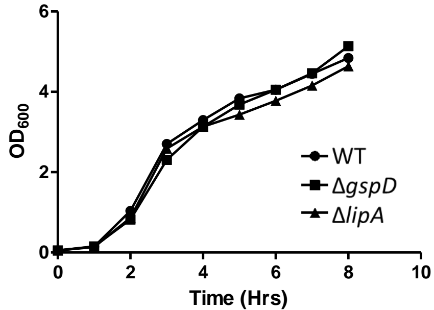
Fig. S1. Deletion of the lipA and gspD genes has no effect on growth in vitro . Overnight cultures were diluted 1:100 and grown in LB broth at 37° C. Growth was monitored over time at 600 nm.
