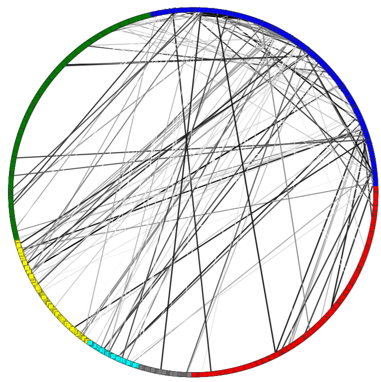
Bond Similarity
