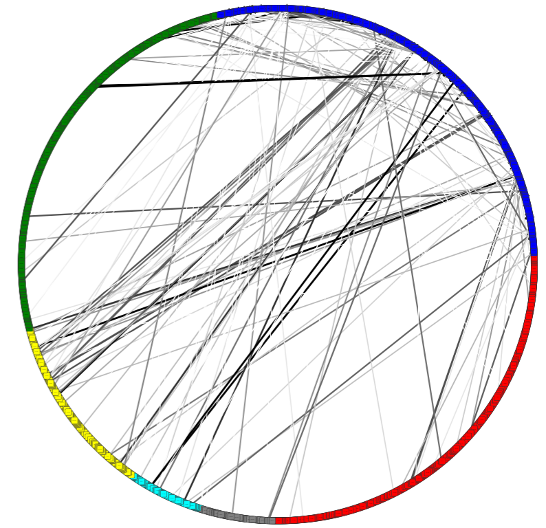
Sub-Structure Similarity
