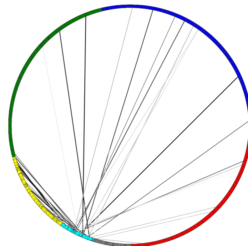
Sub-Structure Similarity
