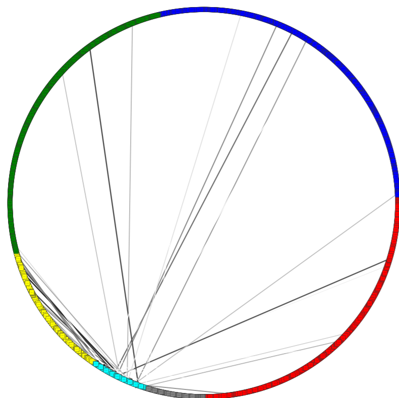
Bond Similarity
