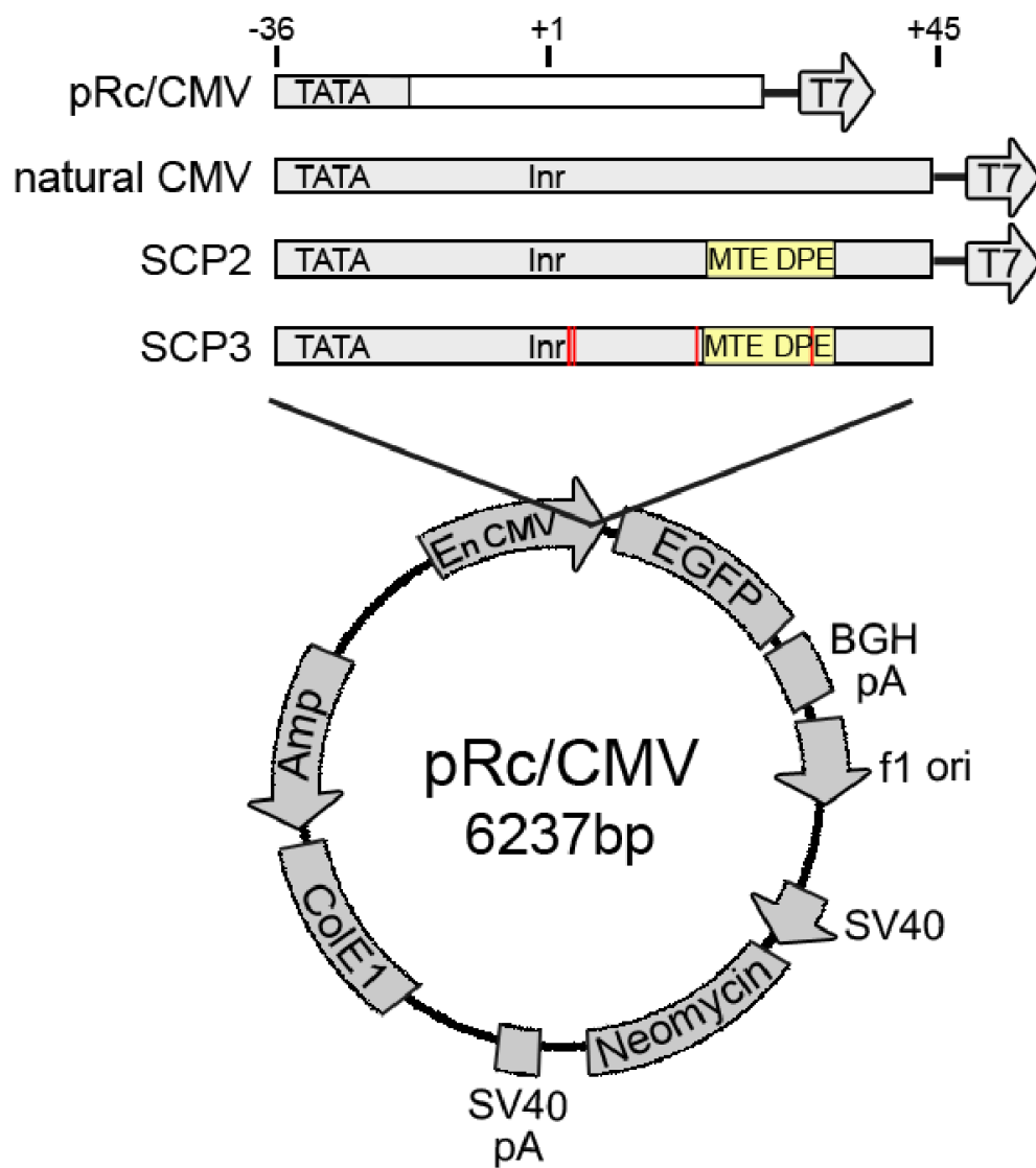
S1 Fig. Schematic illustration of the constructed EGFP expression plasmids driven by the various core promoters linked to the CMV enhancer.
