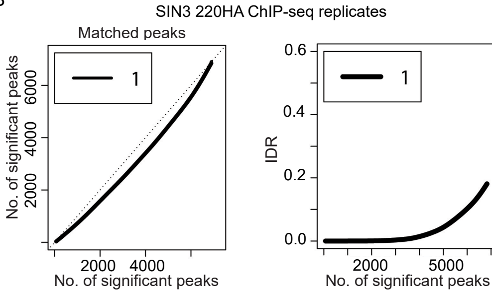
Figure S2. Irreproducible discovery rate (IDR) analysis showing the correlation between the two biological replicates of ChIP-seq analysis for SIN3 187HA samples (A) and SIN3 220HA samples (B). This figure is related to Figure 2, 3.
